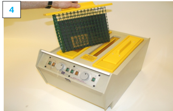
4. Bubble develop exposed plate in Mega Tri-Tank
